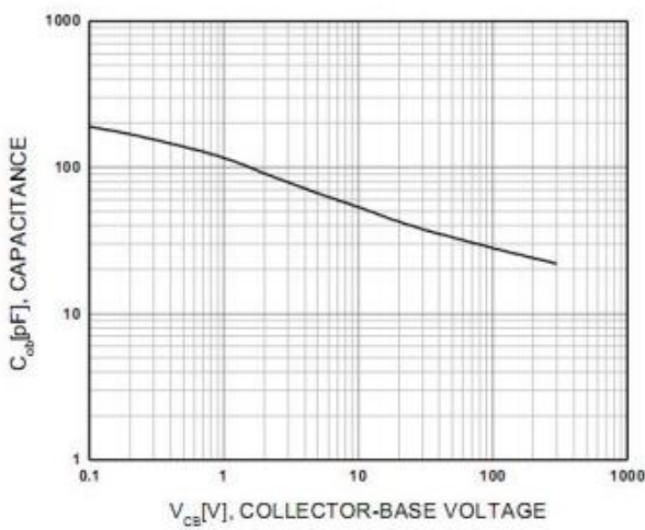
Fig.3 Collector Output Capacitance
