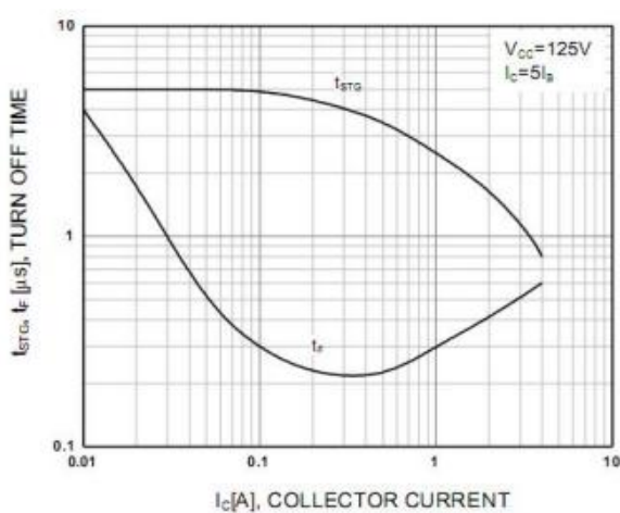
Fig.5 Turn Off Time
