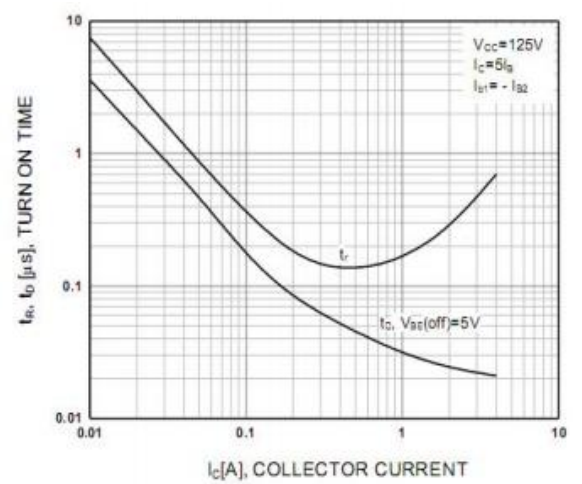
Fig.4 Turn On Time
