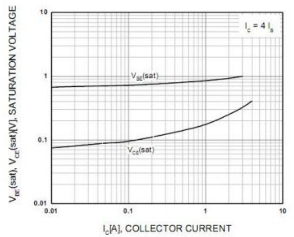
Fig.2 Base-Emitter/Collector-Emitter Saturation Voltage
