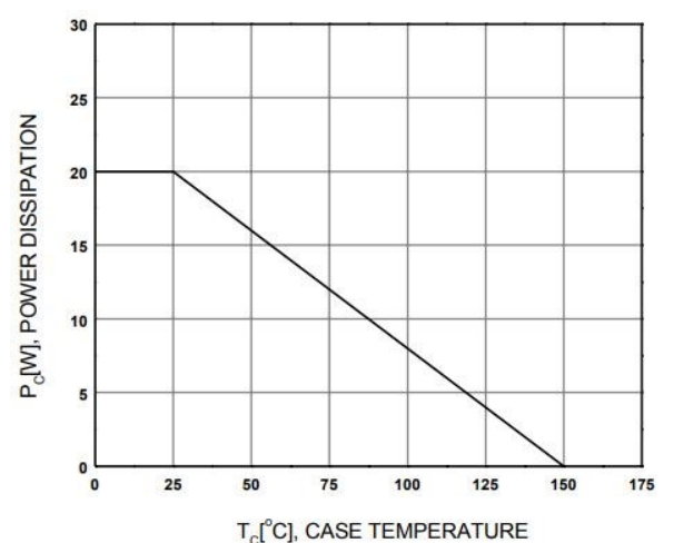
Fig.6 Power Derating
