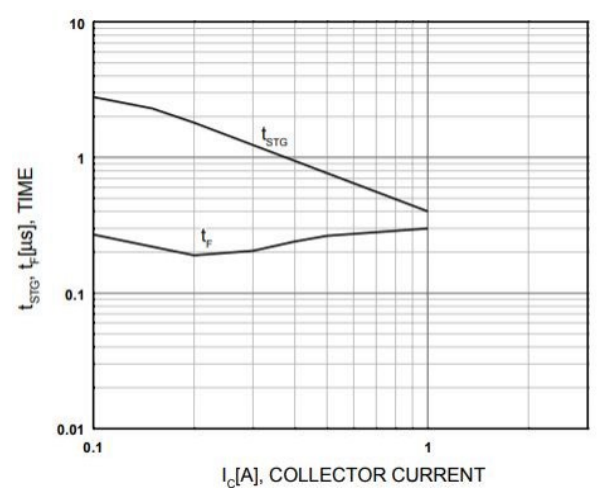
Fig.4 Switching Time
