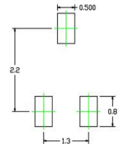
Mounting PAD Layout
