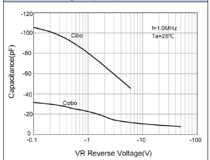
Fig.6 Output Capacitance
