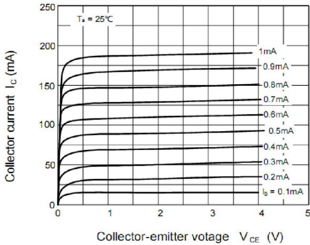
Fig.1 Static Characteristic
