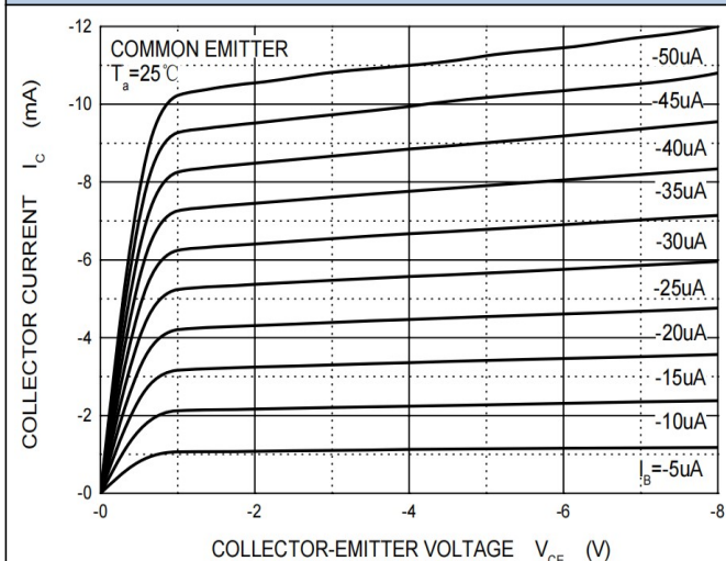
Fig.1 Static Characteristic
