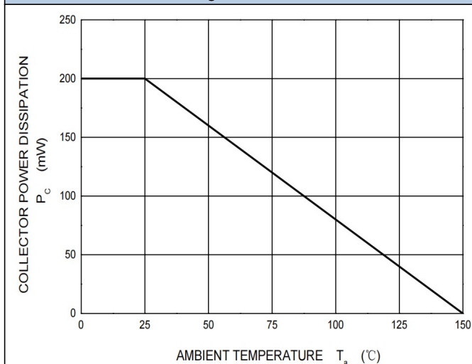
Fig.6 P_C - T_a
