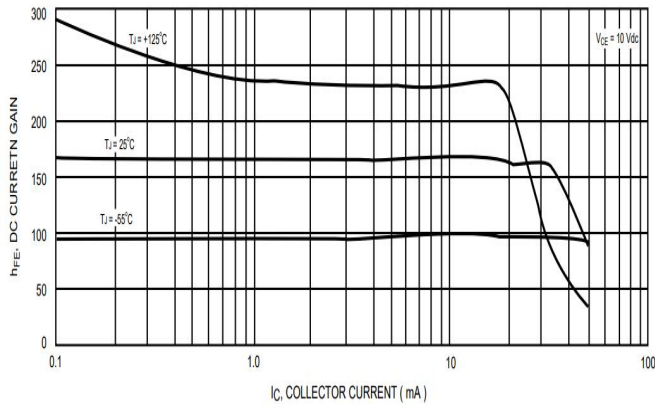
Fig.1 Static Characteristic
