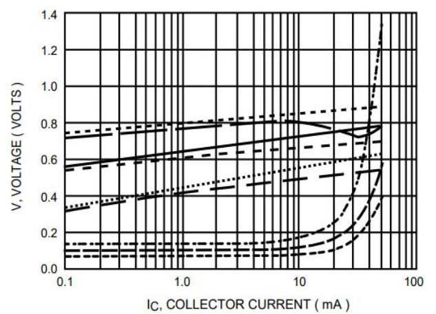
Fig.4 V_{BEsat} \text{ --- } I_C
