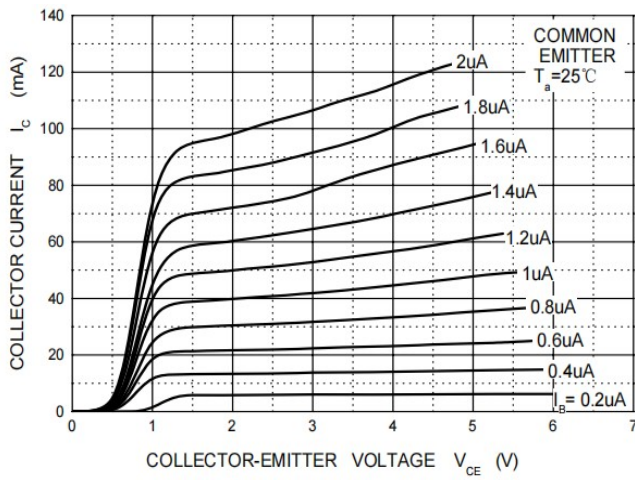
Fig.1 Static Characteristic
