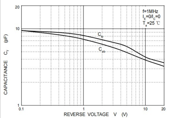
Fig.6 C_{ob}/C_{ib} - V_{CB}/V_{EB}
