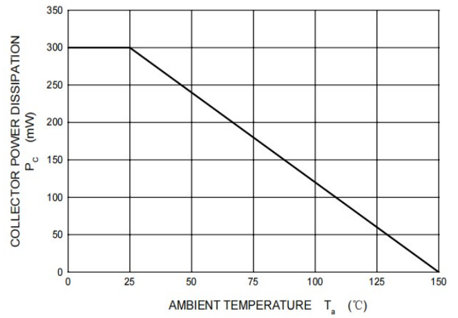
Fig.8 P_C - T_a
