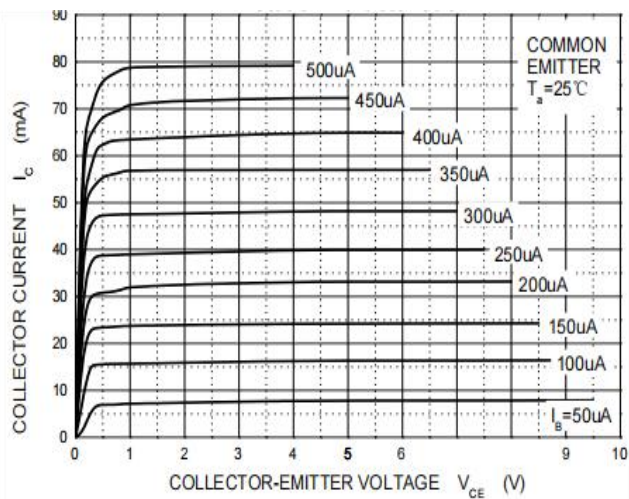
Fig.1 Static Characteristic
