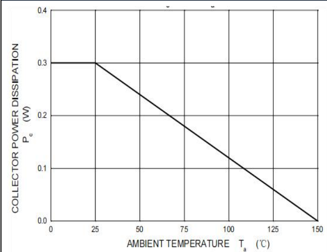
Fig.6 P_c - T_a
