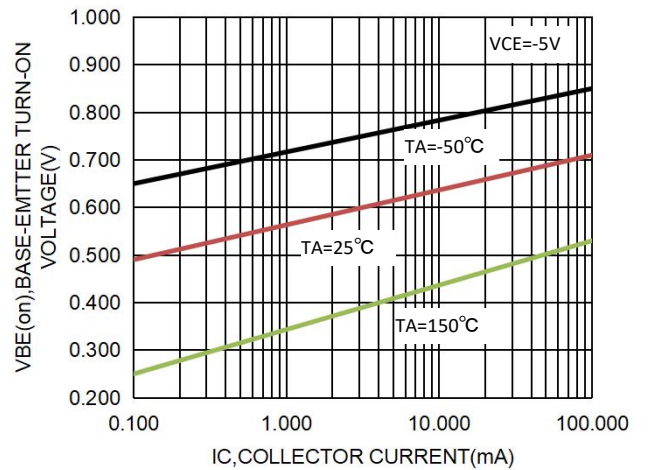
Fig.4 Base-Emitter Voltage vs. Collector Current
