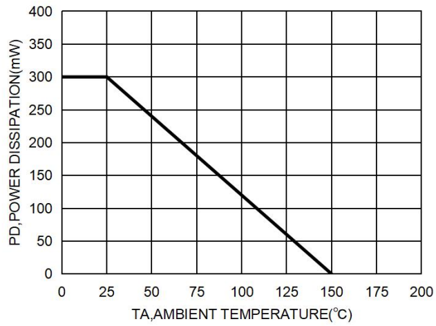
Fig.7 Max Power Dissipation vs Ambient Temperature
