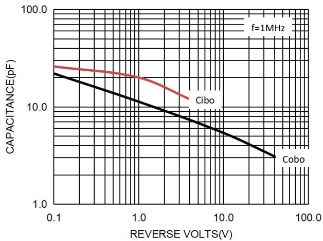
Fig.1 Typical Capacitance
