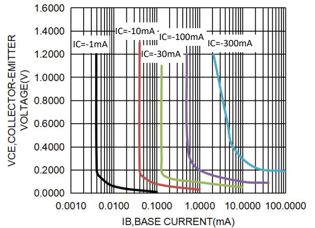
Fig.2 Typical Collector Saturation Region
