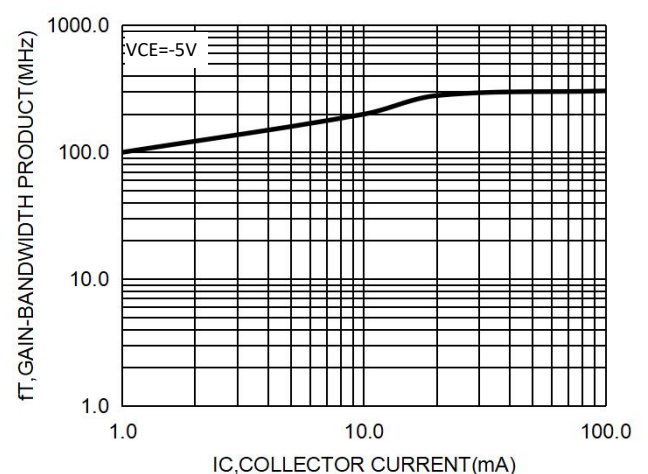
Fig.6 Gain Bandwidth Product vs. Collector Current
