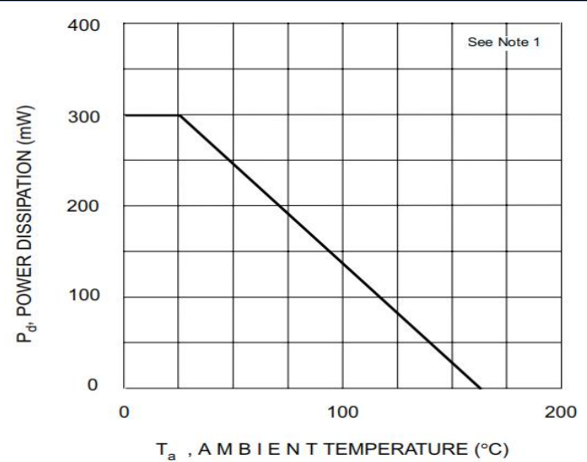
Fig.6 P_C - T_a
