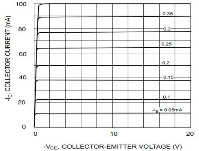
Fig.2 Typical Emitter-Collector Characteristics
