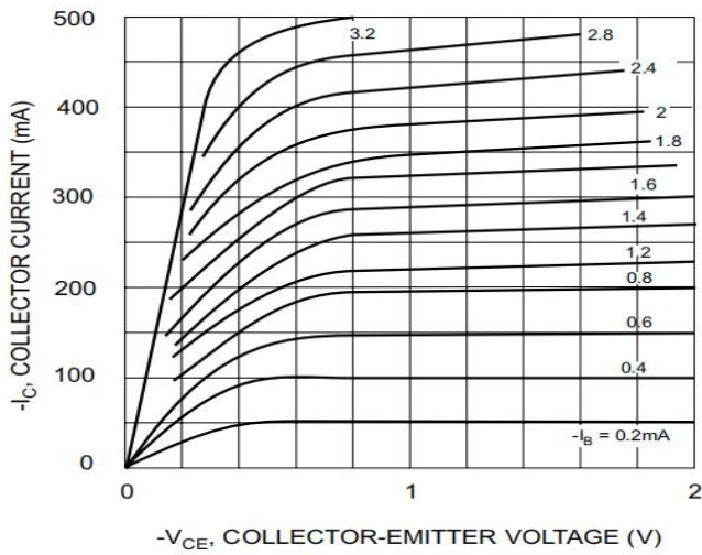
Fig.1 Typical Emitter-Collector Characteristics
