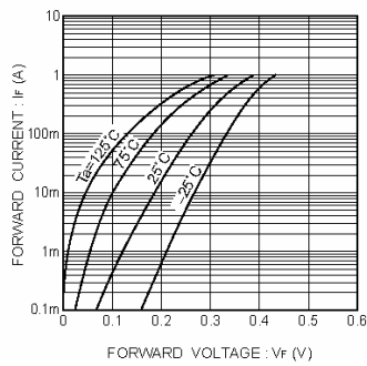
Fig.1 Forward characteristics
