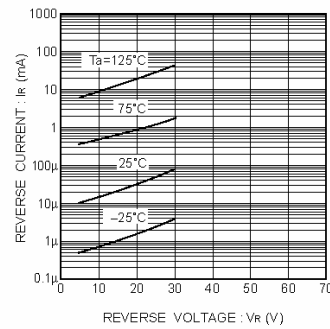
Fig.2 Reverse characteristics
