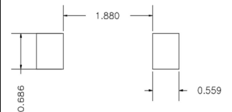
Mounting PAD Layout
