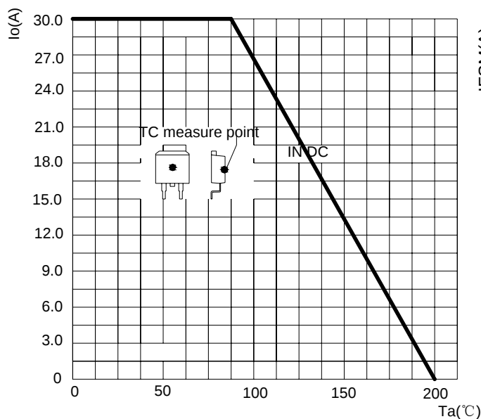
Fig.1: IF(AV)--Tc Derating
