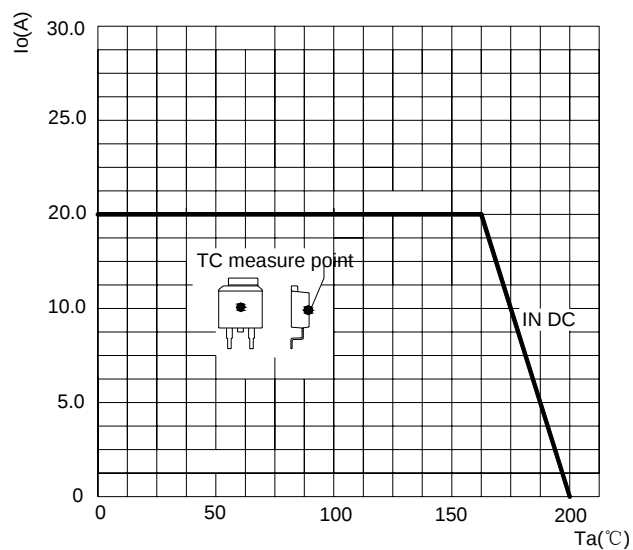
Fig.1: IF(AV)--Tc Derating
