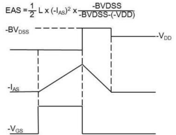
Fig.8 EAS Waveform
