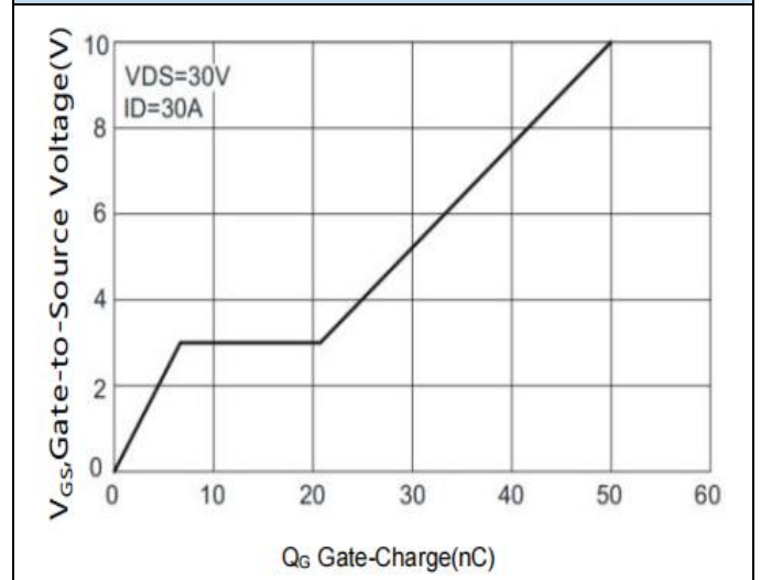
Fig.6 Typical Gate Charge versus V_{GS}
