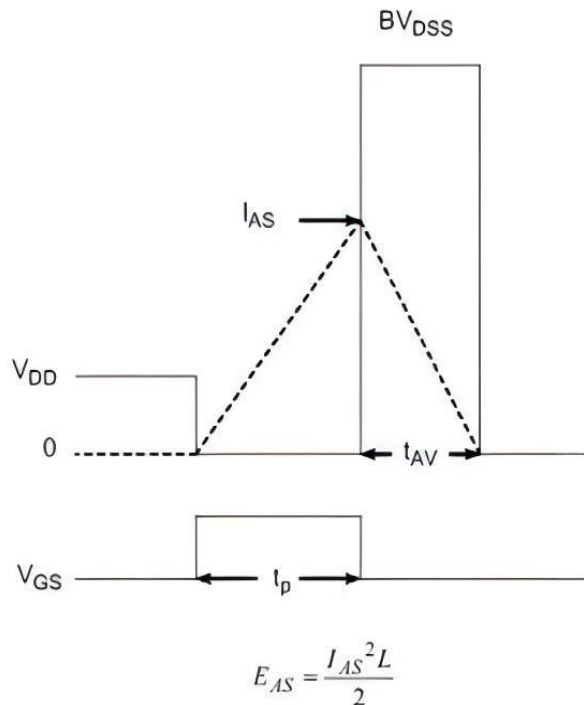
Unclamped Inductive Switching Waveforms
