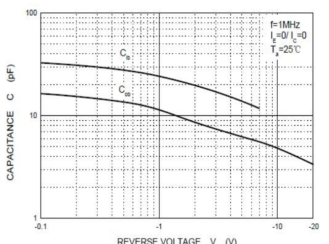
Fig.6 C_{ob}/C_{ib} - V_{CB}/V_{EB}
