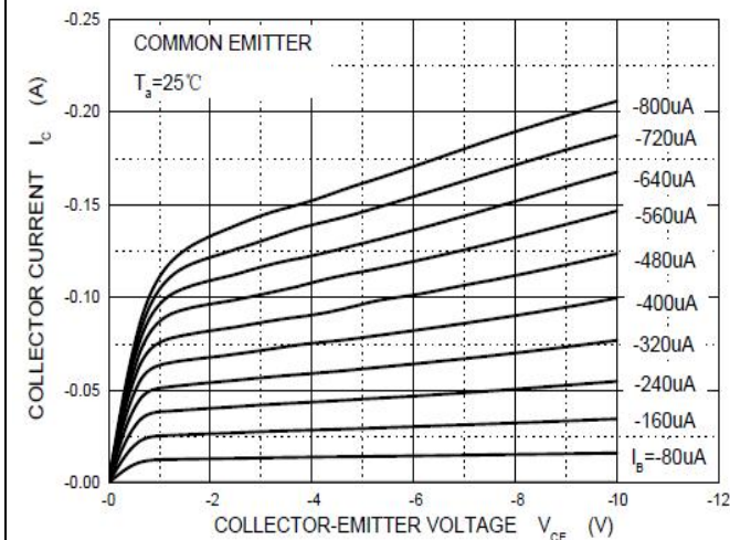
Fig.1 Static Characteristic
