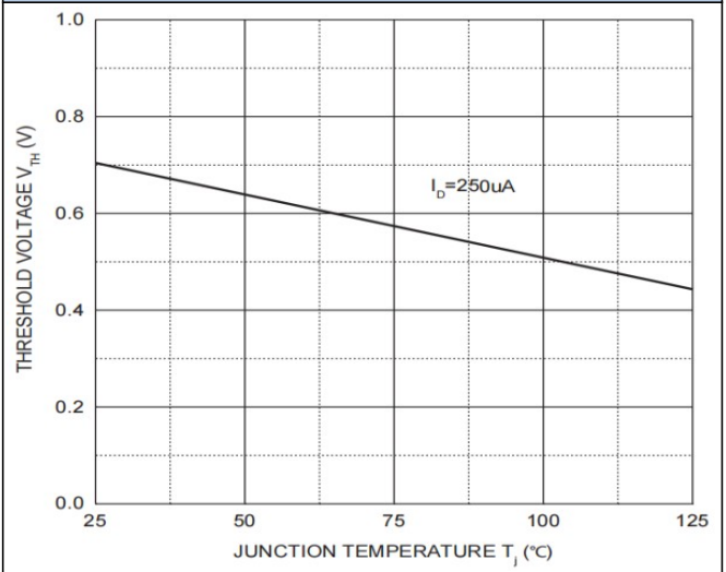
Fig.6 Threshold Voltage
