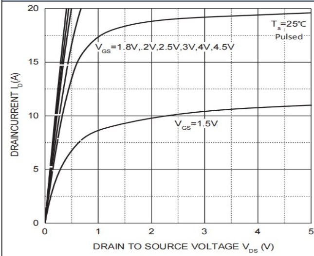
Fig1: Output Characteristics
