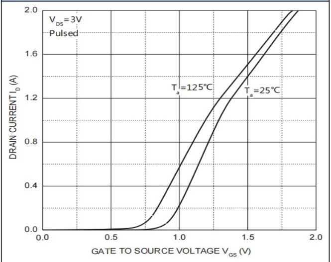
Fig2: Transfer Characteristics
