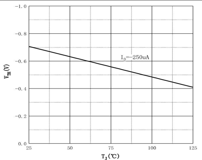
Fig.6 Threshold Voltage
