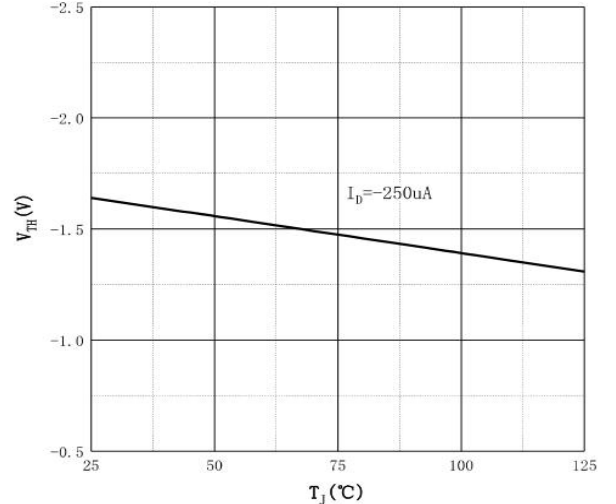
Fig.6 Threshold Voltage
