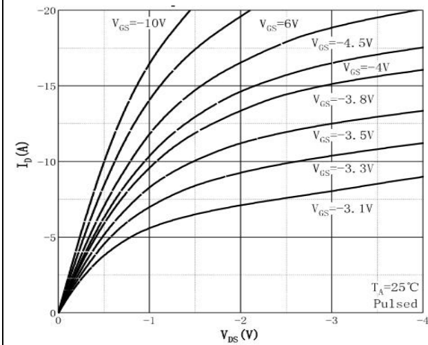
Fig1: Output Characteristics
