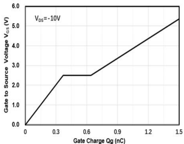
Fig4: Gate Charge
