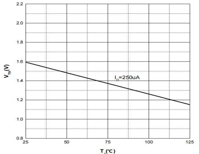
Fig.6 Threshold Voltage
