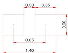
Mounting PAD Layout
