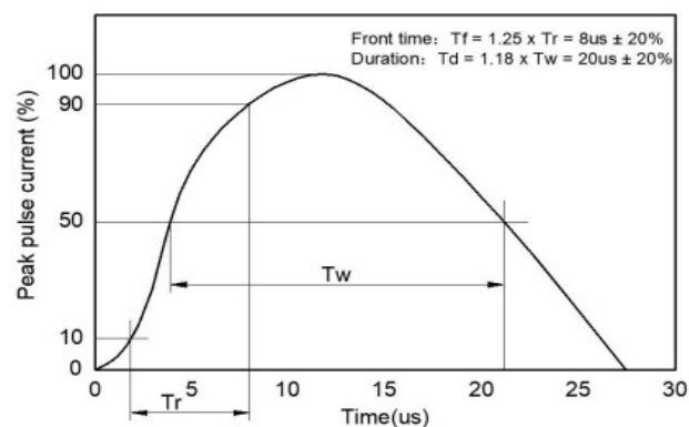
FIG2: pulse Waveform
