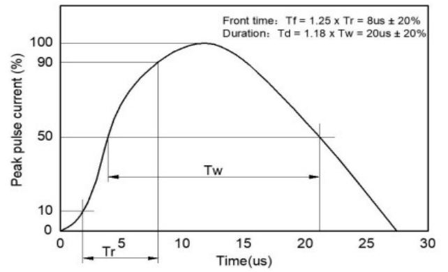
FIG2: pulse Waveform
