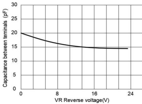
FIG3: Capacitance between
