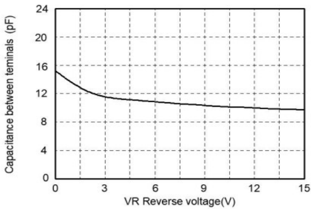
FIG3: Capacitance between
