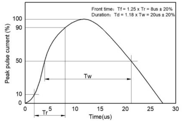
FIG2: pulse Waveform
