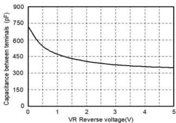
FIG3: Capacitance between teminals charateristics
