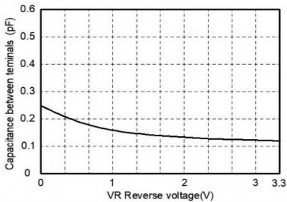
FIG3: Capacitance between
