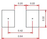
Mounting PAD Layout
