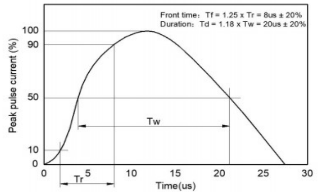
FIG2: pulse Waveform
